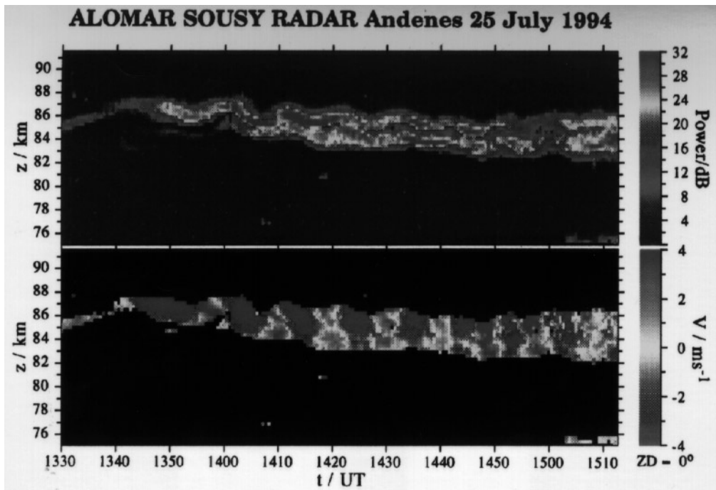
Fig. 1. Height-time intensity plots of the signal-to-noise ratio ( upper part ) and the radial velocity ( lower part ) measured in the vertically pointing beam
