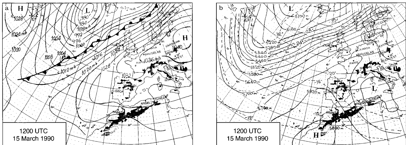
Fig. 2a,b. Synoptic situation at 1200 UTC on 15 March 1990. a Surface analysis (pressure contours every 4 mb); b 500 hPa analysis (height contours, every 60 m, continuous lines ; temperature contours, every 4 °C, dashed lines )
