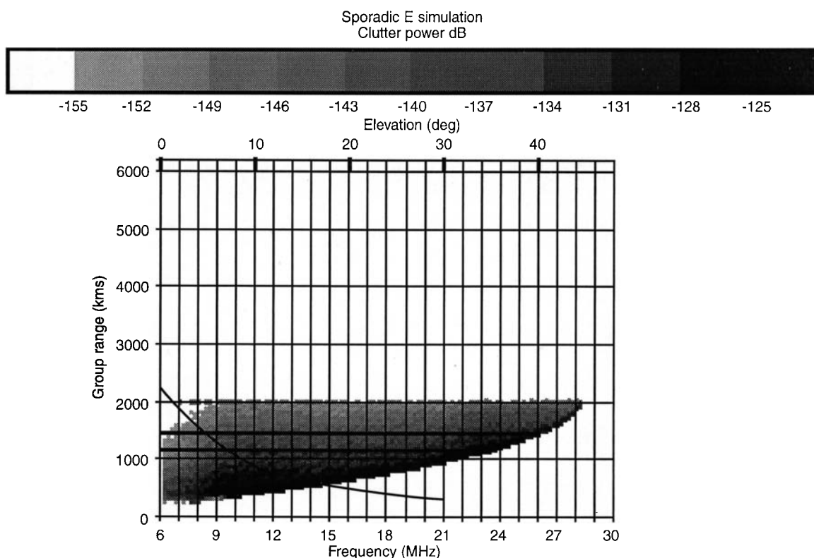
Fig. 3. Backscatter ionogram signature for a single blanketing sporadic-E layer. The curved line shows the variation of elevation angle with group range (scale at top of Fig.). The dark horizontal lines show
