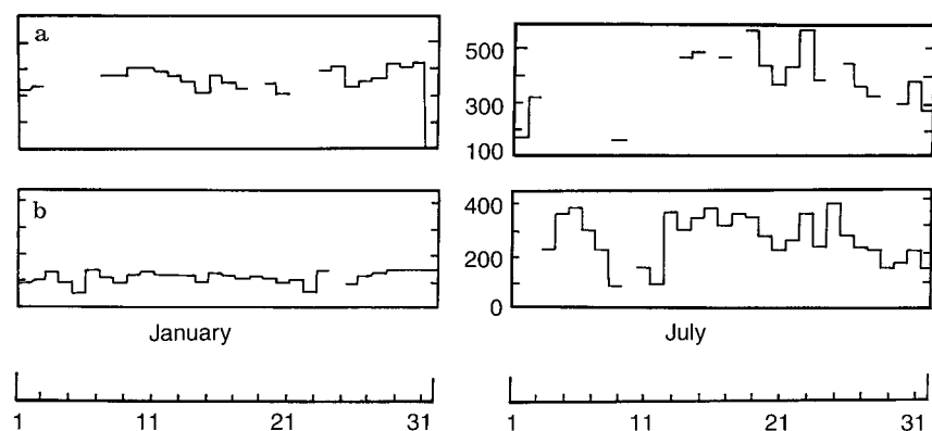
Fig. 3. a Global radiation and b net radiation ( \times 4.186 \times 10^4 ) in January and July at Calcutta in J \cdot m^{-2} \cdot day^{-1}
