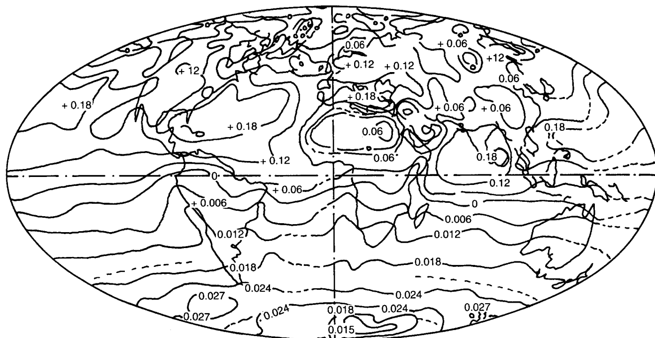
Fig. 1. Radiation balance of the Earth-atmosphere system for July over the entire path (after Raschke et al. , 1967). The figure indicates
