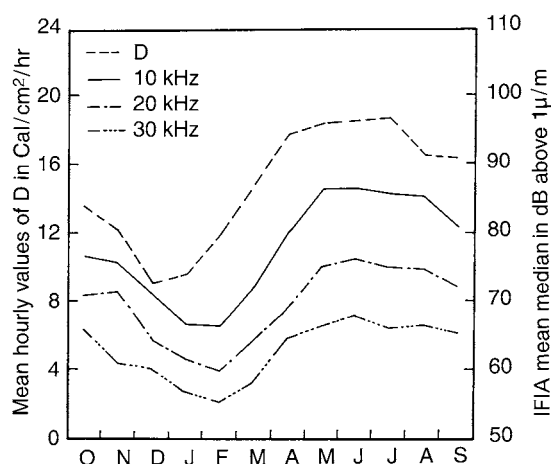
Fig. 5. Mean hourly values of diffuse radiation and median IFIA plotted month by month
