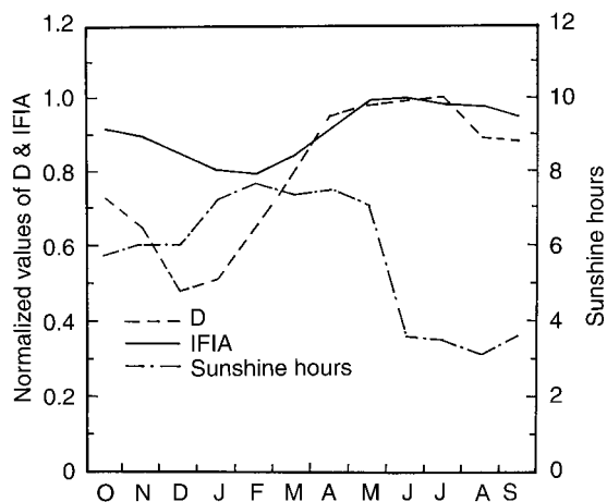
Fig. 7. Curves showing the sunshine hours, and normalized values of (1) diffuse radiation and (2) IFIA for Calcutta
