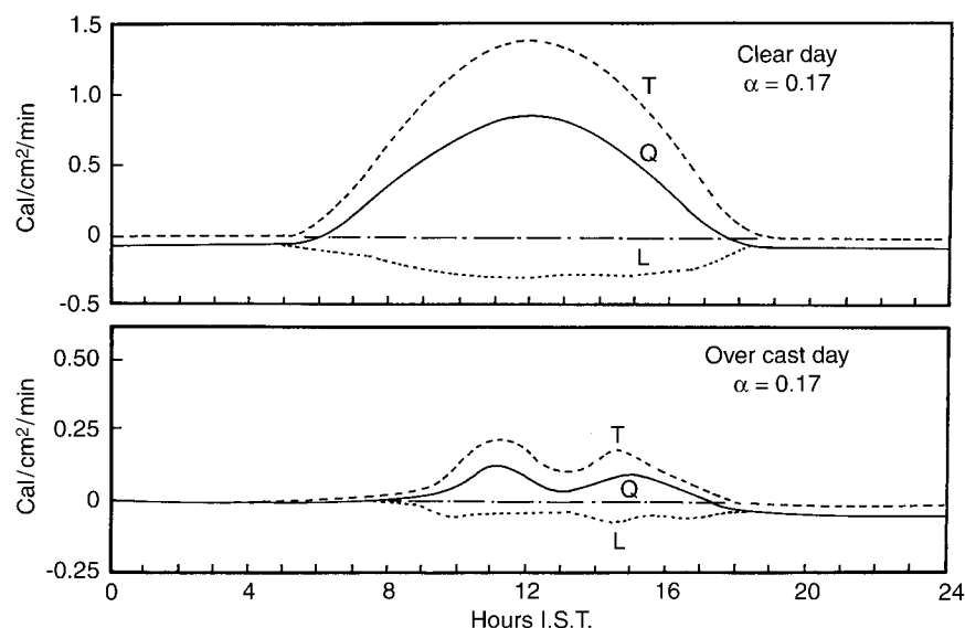
Fig. 2. Global radiation ( T ), net radiation ( Q ) and net terrestrial radiation ( L ) at Calcutta in Indian Standard Time (IST). The data plotted along the Y-axis is to be multiplied by 4.186 \times 10^4 to represent the values in J \cdot m^{-2} \cdot min^{-1}
