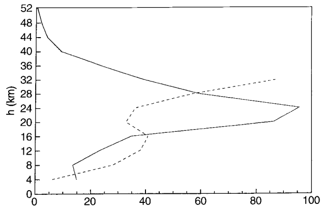
Fig. 3. 24 December 1992; solid line: O_3 profile ( 10^{11} molecules cm^{-3} ); dashed line: zonal velocity profile ( 0.5 \text{ m s}^{-1} )
