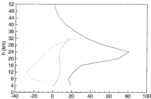
Fig. 11. 5 December 1993; solid line: \text{O}_3 profile ( 10^{11} molecules \text{cm}^{-3} ); dashed line: zonal velocity profile ( 0.5 \text{ m s}^{-1} ); dotted line: meridional velocity profile ( 0.5 \text{ m s}^{-1} )
