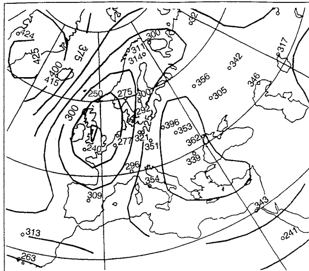
Fig. 5. 6 March 1993; ozone map (Courtesy of LAP Univ. of Thessaloniky, Greece)
