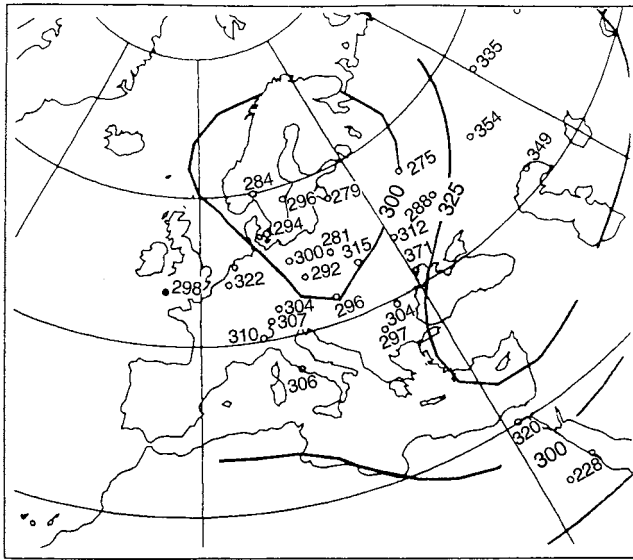
Fig. 1. 24 December 1992; ozone map (Courtesy of LAP Univ. of Thessaloniky, Greece)
