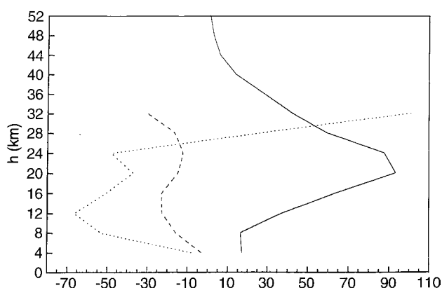
Fig. 7. 6 March 1993; solid line: O_3 profile ( 10^{11} molecules cm^{-3} ); dashed line: zonal velocity profile ( 0.5 \text{ m s}^{-1} ); dotted line: meridional velocity profile ( 0.5 \text{ m s}^{-1} )
