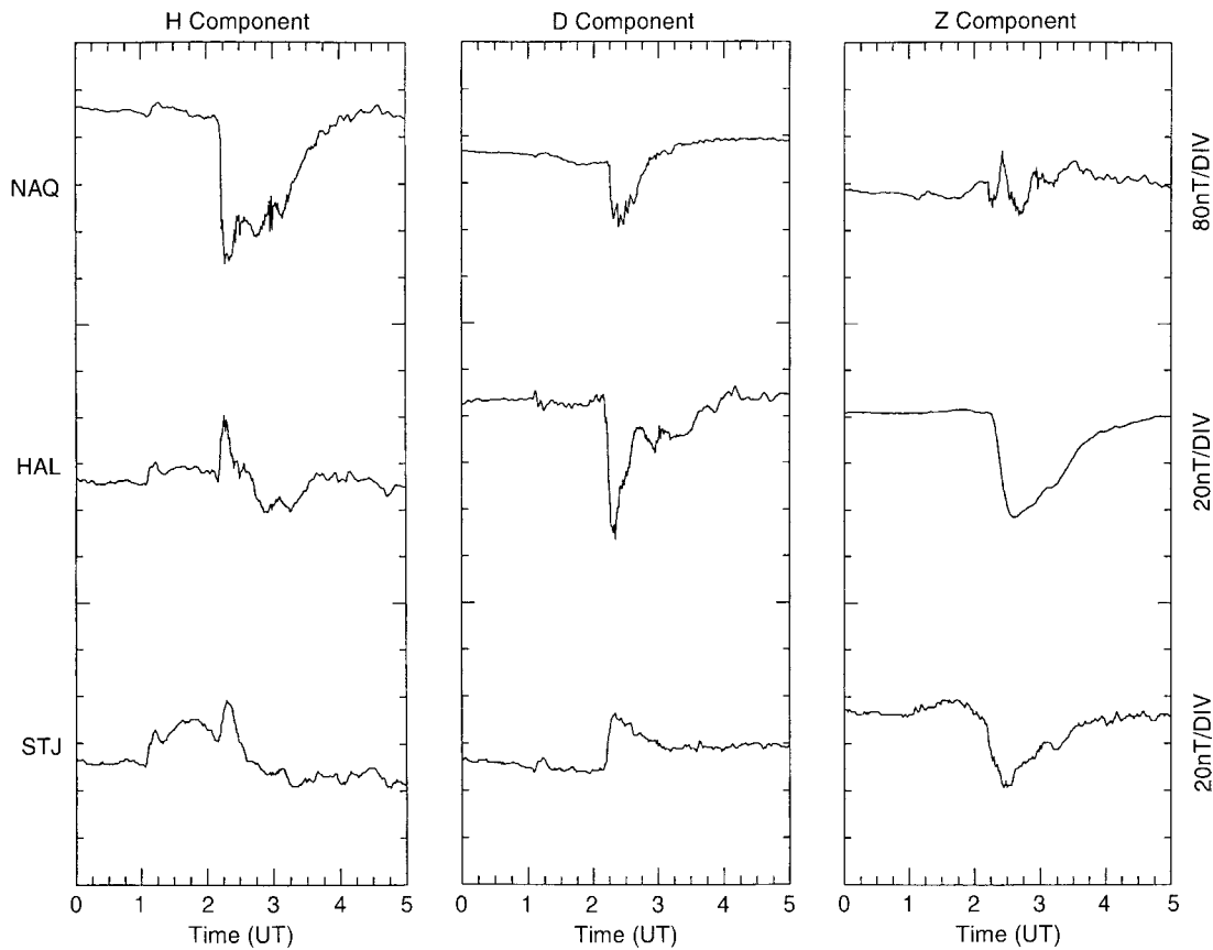
Fig. 4. Stacked magnetograms of the H, D, and Z components from Narssarssuaq (NAQ), Halley (HAL) and St Johns (STJ) between 00:00 UT and 05:00 UT on 13 June 1988. Note the different scale for NAQ. The data are in local magnetic coordinates where the quiet-
