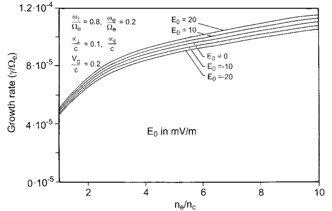
Fig. 5. Variation of growth rate ( \gamma/\Omega_e ) with n_e/n_c for \alpha_{\perp}/c = \alpha_{\parallel}/c = 0.1 , v_0/c = 0.2 , \omega_e/\Omega_e = 0.2 , and for different values of E_0 = 0, 10, 20 mV/m
