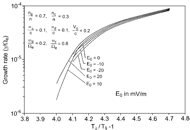
Fig. 3. Variation of growth rate ( \gamma/\Omega_e ) with (T_{\perp}/T_{\parallel} - 1) for \omega_e/\Omega_e = 0.2 , \alpha_{\parallel}/c = \alpha_{\perp}/c = 0.1 , v_0/c = 0.2 , n_c/n_c = 0.7 , and for different values of E_0 = 0, 10, 20 mV/m
