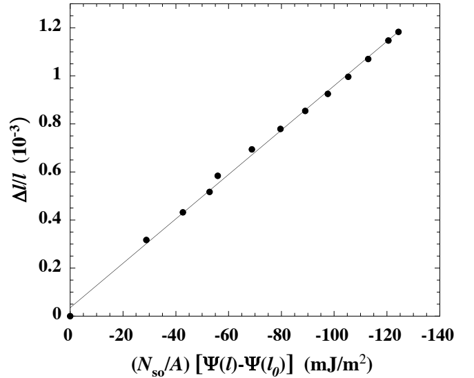
FIG. 3: Linear extension ( \Delta l/l ) of a porous glass rod measured by Amberg and McIntosh (Ref. 24 ) during water adsorption at 18.75°C as a function of (N_{\text{so}}/A) [\Psi(l) - \Psi(l_0)] , where N_{\text{so}} is the total number of solid atoms, A , the surface area and [\Psi(l) - \Psi(l_0)] , the variation of the "effective" surface free energy per solid atom as defined in Eq. (15) and calculated according to Eq. (19). l_0 is the length of the porous rod before adsorption. The surface area equals 129 m 2 /g. The regression coefficient of the linear fit equals 0.999.
