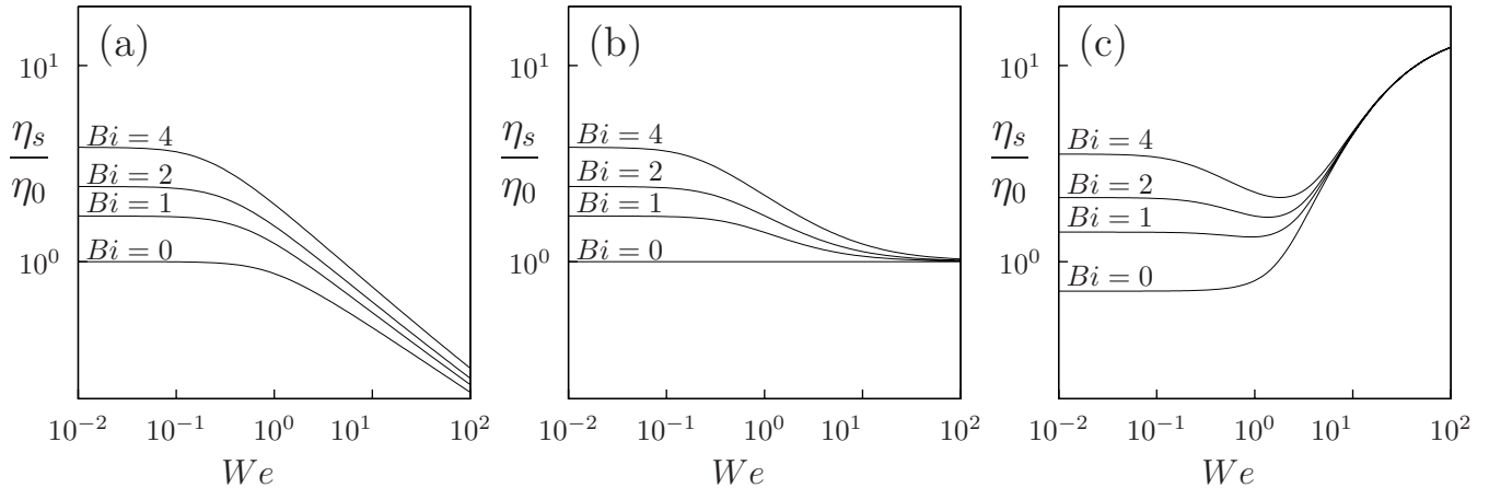
Figure 6: Steady shear viscosity for a = 1 , \alpha = 1 and (a) n = 0.5 ; (b) n = 1 ; (c) n = 1.5 .
