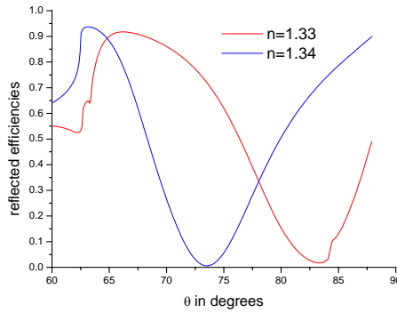
Fig. 9. Reflected efficiency as a function of the angle of incidence \theta . h_1=35 nm, h_2=59 nm, t=40 nm, \varphi=\pi/2 .
