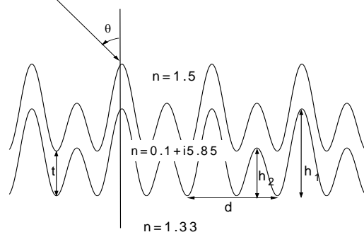
Fig. 6. Same as Fig. 1 with a second periodical modulation of height h_2 .
