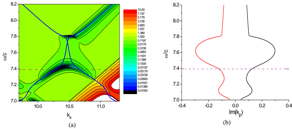
Fig. 10. (a) Colour map dependence of the intensity of the 0th reflected order of a single-harmonic grating with h_1 = 20 \text{ nm} ( h_2 = 0 ). Thick blue lines, real part of the constant of propagation of the plasmon surface waves excited on the substrate-metal layer interface. Purple line, working point at \lambda = 0.85 \mu\text{m} . (b) Imaginary parts of the surface waves propagation constants as a function of \omega/c .
