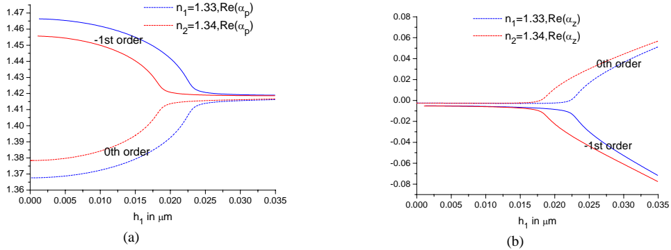
Fig. 3. Similar to Fig. 2 with the zeros satisfying eq.(2).
