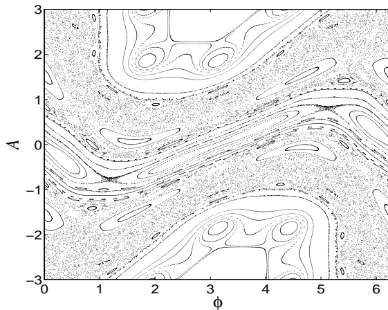
Fig. 3. Phase portrait of the controlled standard map S_{\text{mix},2} with the control term (16) for \varepsilon = 1.2 .
