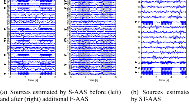
Figure 2: Estimated sources by S-AAS and ST-AAS, Fig. 2(a) and 2(b), respectively. Note that each source is normalized separately to have a unit standard deviation so they do not have the same ordinate axis. The gray plots are the estimated sources before the additional F-AAS algorithm.
