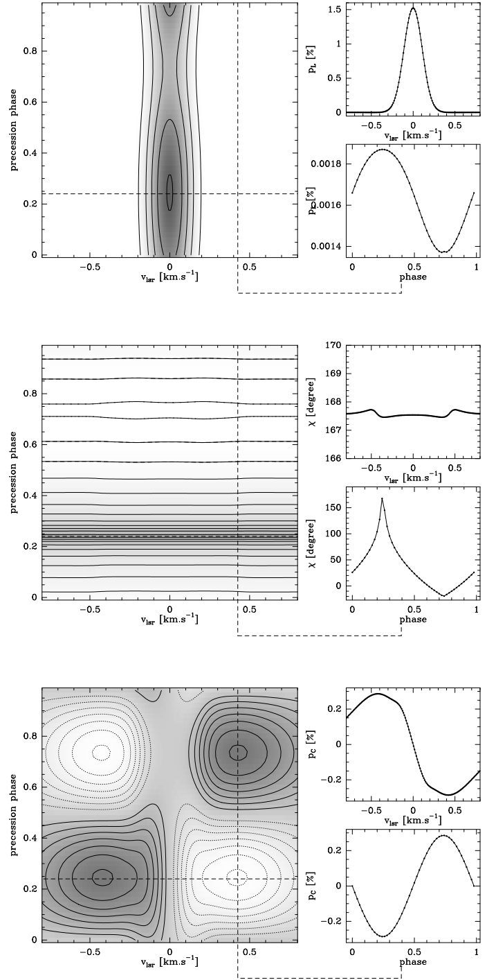
Fig. 6. Same as Fig. 4, but 3 r_J above the planet's equatorial plane and towards its rotation axis (model 2c). Top: p_L , contour levels 0.3 % to 1.5 % by 0.3 %. Center: \chi , contour levels from -16^\circ to +160^\circ by 16^\circ . Bottom: p_C , contour levels from -0.28 % to +0.28 % by 0.04 %.
