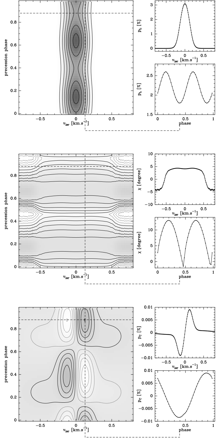
Fig. 4. Unsaturated SiO maser ( I_{\text{peak}} = 0.1 I_S ), pencil beam at r = 3 r_J , in the planet's equatorial plane (model 2a). The linewidths are narrowed with respect to the thermal width, as expected for unsaturated maser action. Top: p_L , contour levels from 0.6% to 4.2% by 0.6%. Center: \chi , contour levels -12^\circ to 12^\circ by 3^\circ . Bottom: p_C , contour levels from -0.009\% to +0.009\% by 0.002\% .
