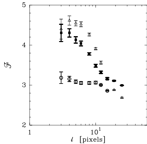
Fig. 7. Flatness \mathcal{F} of the CVI (see Eq. (2)) computed from the normalized PDF of CVI. Squares : Polaris ^{12}\text{CO}(1-0) IRAM data. Triangles : ^{12}\text{CO}(2-1) KOSMA data. Circles : Taurus ^{12}\text{CO}(1-0) IRAM data.
