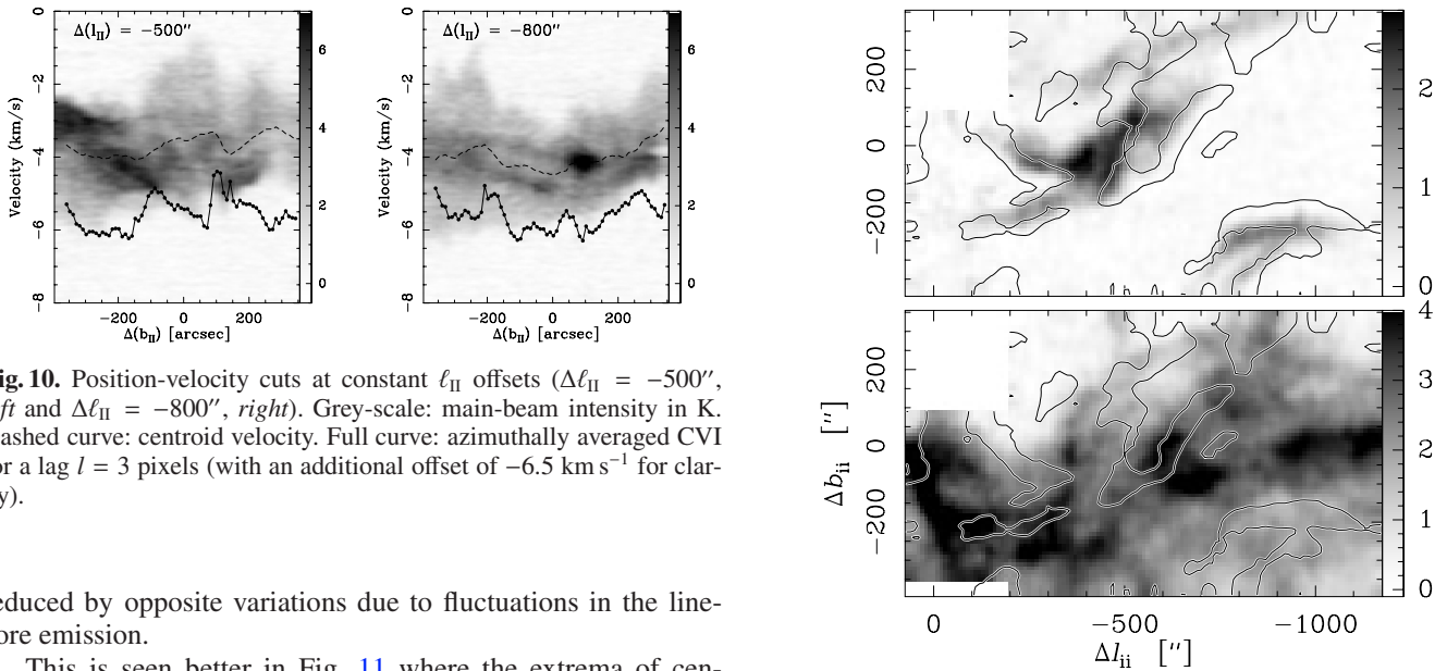
Fig. 11. Contours of the CVI ( 1 \text{ km s}^{-1} ) computed in the Polaris field for l = 3 pixels (see Fig. 9) overplotted on the ^{12}\text{CO}(1-0) emission integrated in the velocity range [-2, 5:0] \text{ km s}^{-1} i.e. optically thin ^{12}\text{CO} emission (top) and the ^{13}\text{CO} integrated intensity tracing the bulk of the dense gas (see Paper II) (bottom).
