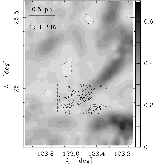
Fig. 12. Spatial distribution of CVI ( \text{km s}^{-1} ) computed on large scales using the data of Bensch et al. (2001) (grey-scale with levels indicated on the right scale, dotted contours indicate the 0.1 \text{ km s}^{-1} level). Full-line contours indicate the CVI computed on small scales in the IRAM-30 m data cube (see Fig. 11). Note the spatial coincidence of the IRAM structures at the tip of the prominent KOSMA structure at (123.4°, 25°), where the CVI are 0.30 \text{ km s}^{-1} .
