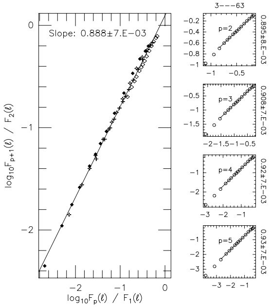
Fig. A.4. The \alpha -test to both the Polaris field (see Appendix A.3) where \alpha = \beta^\theta with \theta = 1/3 . All orders are plotted on the left panel and fitted with a single power law, while the right panels detail the fits to individual orders p = 2, 3, 4, 5 . Fits are done over the range indicated by the line. The individual slopes are 0.90, 0.91, 0.92 and 0.93.
