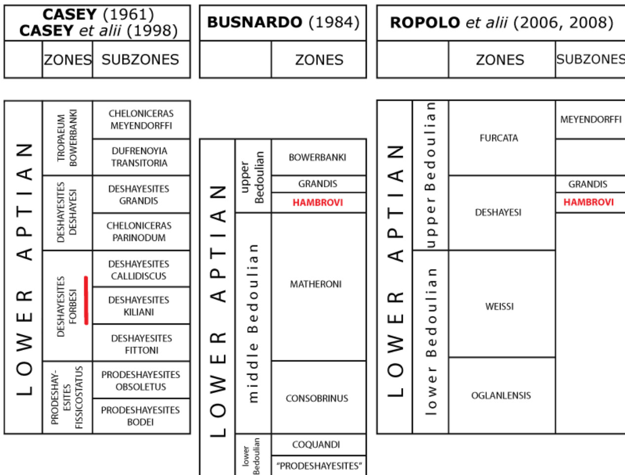
Figure 4: Correlation between the Lower Aptian ammonite zonations of CASEY (1961a, 1998), BUSNARDO (1984) and ROPOLO et alii (2006, 2008).
