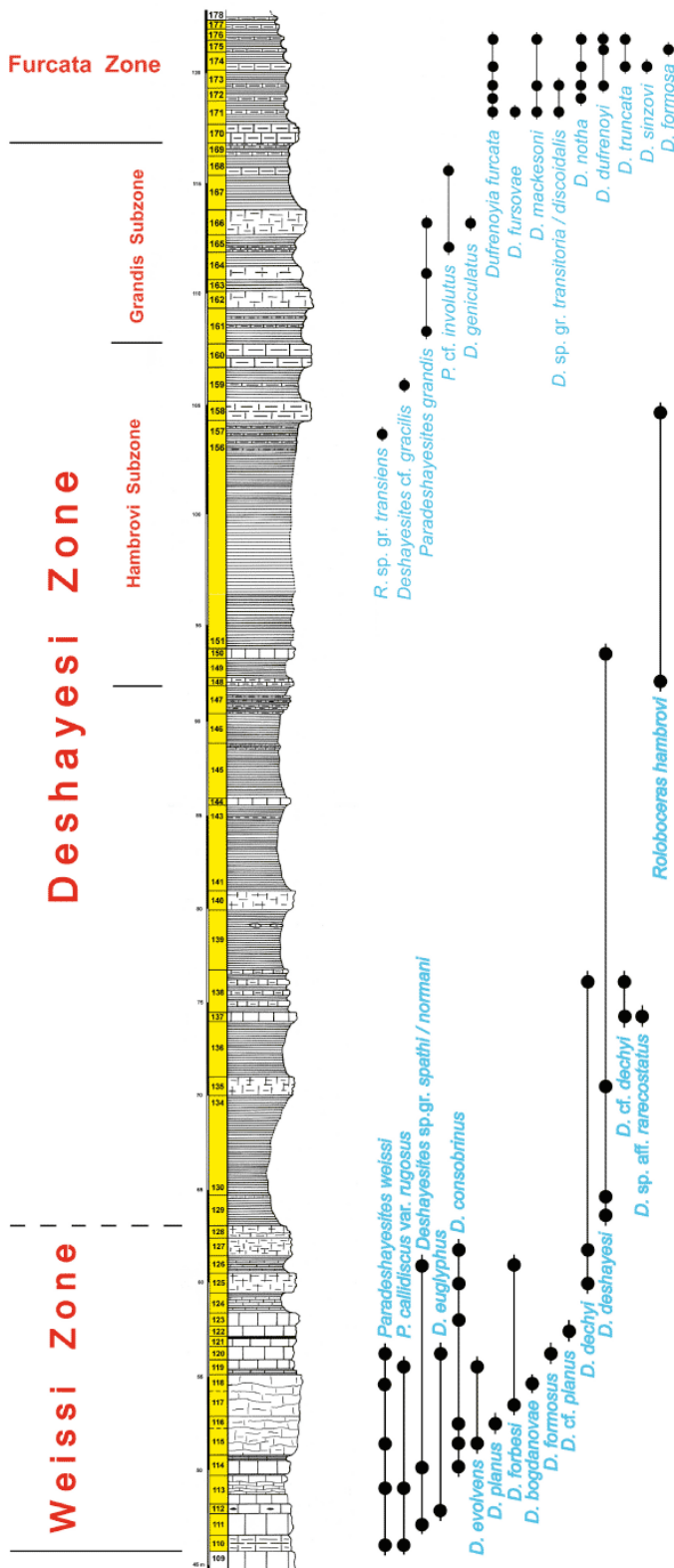
Figure 3: Cassis-La Bédoule railway station section: stratigraphic range of the Deshayesitidae and Roloboceratinae (from ROPOLLO et alii , 2006).
