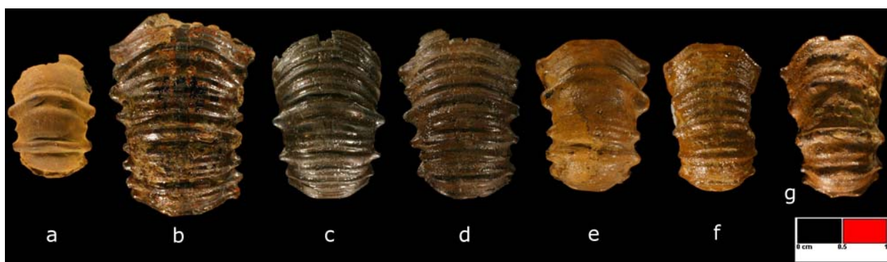
Figure 9: (from left to right): evolution of Chelonicerias cornuelianum towards Epicheloniceras . a) Chelonicerias royerianum (lowermost Dufrenoyia furcata Zone); b-d) Chelonicerias cornuelianum ( Dufrenoyia furcata Zone); e-f) transitional forms to the genus " Epicheloniceras " and appearance of ventral tubercles = Epicheloniceras martini "ex-gr. occidentalis " (JACOB) (lowermost Epicheloniceras martini Zone); g) Epicheloniceras martini martini (d'ORBIGNY) = Epicheloniceras martini ex-gr. " orientalis " (JACOB) ( Epicheloniceras martini Zone) [Photographs A. ARNOUX].
