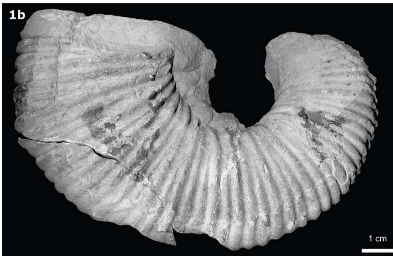
1.a-b) Epicheloniceras gracile CASEY, La Bédoule, probably La Marcouline quarry section, undetermined bed, DEROGNAT Collection, labeled D10.
