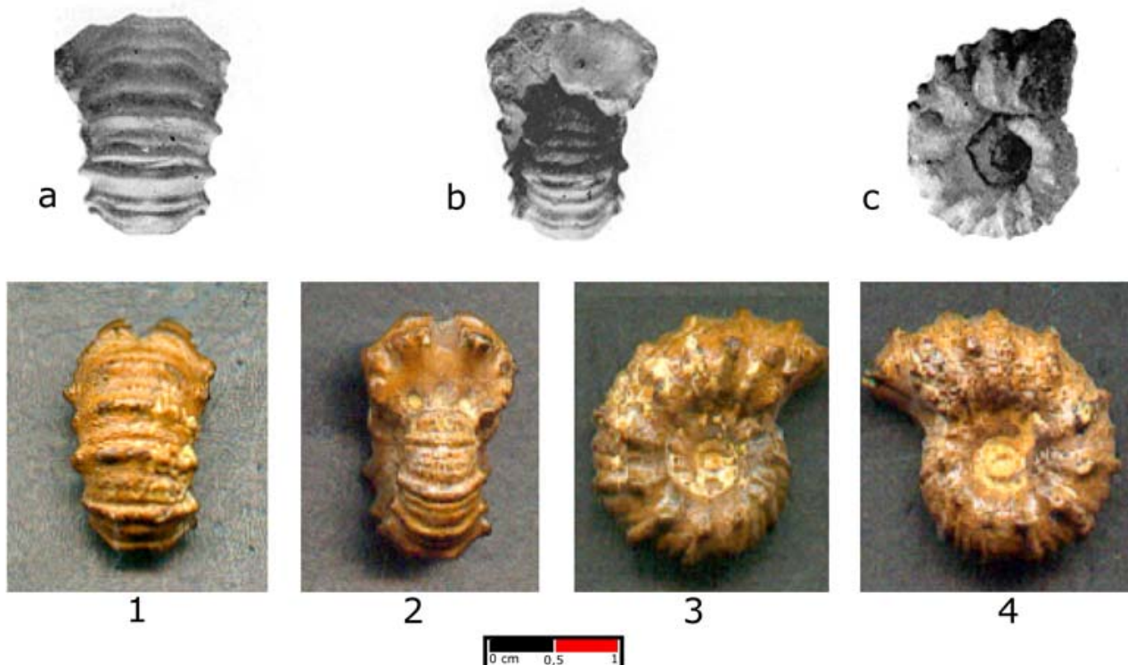
Figure 13: a-c: Epicheloniceras martini "orientalis" JACOB, in KUDRIAVTSEV 1960, Pl. XXI, figs. 2.a-c (venter still flat and wide as in Chelonicerias cornuelianum ) – 1-4: Epicheloniceras martini (d'ORBIGNY), four views of the same specimen, La Marcouline Quarry section (venter rounded; this is the final stage of E. martini ).
