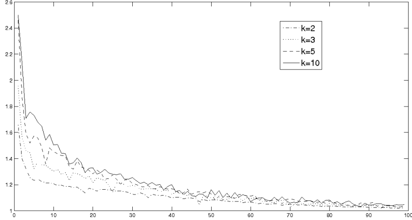
Figure 8: Ratio R_{mer} versus \sigma for different values of k for the meronymy relationship. Similar conclusions can be drawn than in fig 7.
