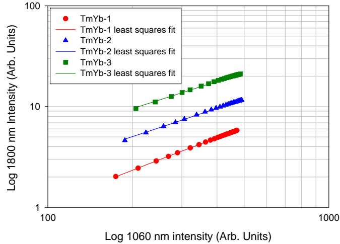
Fig. 3. Log/log plot of the 1800 nm luminescence from \text{Tm}^{3+} vs. the 1060 nm luminescence from \text{Yb}^{3+} , for incident pump powers ranging from 3 - 108 mW. The 1800 nm measured data have been offset to aid comparison. Note: the errors associated with these measurements are not shown as they are smaller than the size of the individual data points in the plot.
