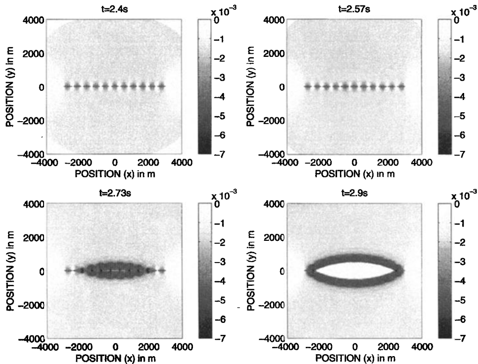
Figure 5. (top) The \gamma parameter at the end of the initiation process and at the beginning of rupture propagation. Note the change of \gamma with time at a given point.
