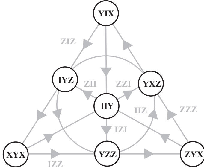
Figure 3: The oriented dual Fano plane.
