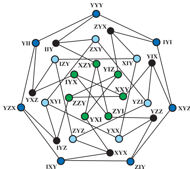
Figure 5: The Coxeter graph, in a form showing its automorphism of order seven, as a subgraph/subgeometry of the Hexagon (see Fig. 4).
