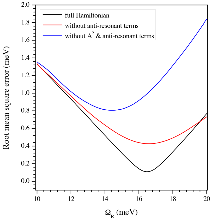
FIG. 8: Supplementary material of arXiv:0808.3720. (a) Root mean square deviation from the measured dispersion of the calculated polariton energies as function of the vacuum Rabi energy, the lone fitting parameter. The red curve refers to the case of no H_{anti-res} terms, while the blue to the case without both H_{dia} and H_{anti-res} contributions. The black line is for the full Hamiltonian. The values corresponding to minima of each curve have been used to compute the polariton dispersions in Fig. 3 of the paper.
