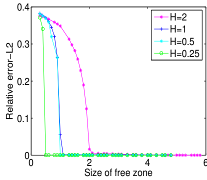
Figure 3b. Relative discrete L^2 errors versus the the size of S_f^{01}
