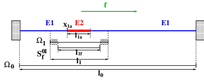
Figure 2a. A single alteration
