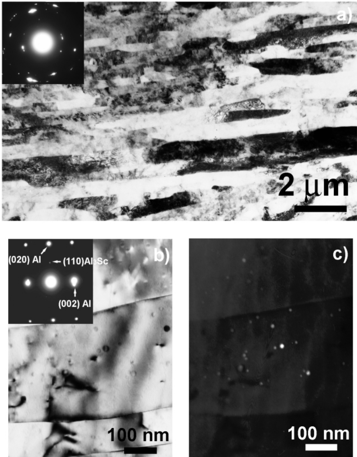
Figure 6: TEM images of the bulk microstructure of the AlMgSc alloy. (a) Low magnification bright field image showing the typical microstructure of the rolled sheet (rolling direction is horizontal) and corresponding SAED pattern (aperture diameter 5 μm). (b) High magnification bright field image (SAED, aperture diameter 0.4 μm) and (c) corresponding dark field image obtained by selecting the (200) lattice reflection and showing nanoscaled precipitates.
