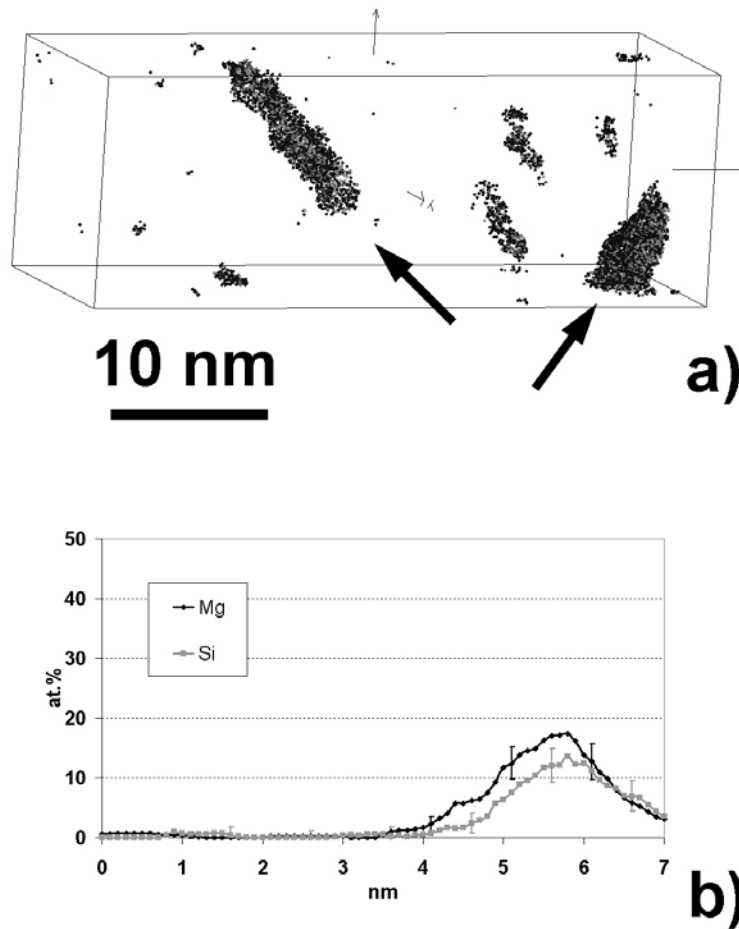
Figure 3: Three-dimensional atom probe data set collected in the bulk AlMgSi alloy ( 15 \times 15 \times 40 \text{ nm}^3 ). (a) Filtered data : only Al, Mg and Si atoms within regions containing at least 7at.% Mg are displayed to exhibit two orthogonal needle shaped precipitates (iso-position procedure). (b) Composition profile computed across a needle shaped precipitate (sampling box thickness is 1 nm).
