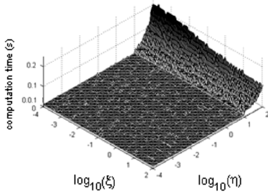
Fig. 7. Computation time for J_{\text{alg2}}(\eta, \zeta, 0) .
