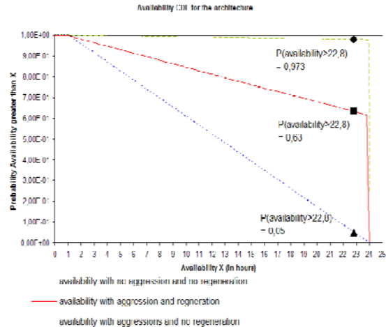
Figure 11 – Availability CDF of the architecture
