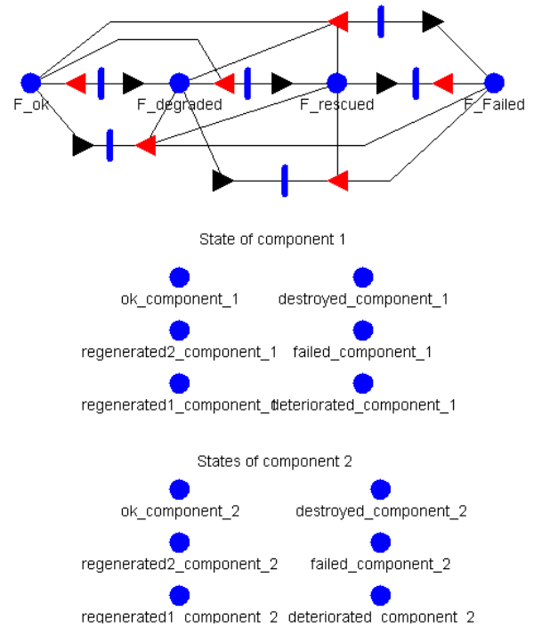
Figure 8 – SAN function model
