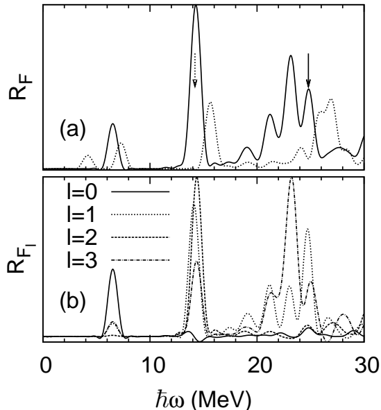
FIG. 2: Decomposition of the responses (in arbitrary units) into frequencies \omega for a two-neutron pair transfer excitation in ^{18}\text{O} . (a) Strength distribution of \hat{F} obtained from TDHFB (solid line) and the unperturbed approximation (dotted line). The arrows indicate the 1p_{3/2} (solid) and 1p_{1/2} (dotted) deep hole states. (b) TDHFB responses of \hat{F}_l with l = 0, 1, 2 and 3 .
