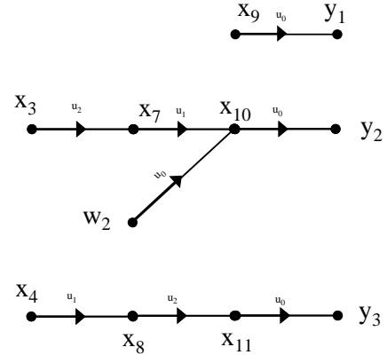
Figure 2. A -disjoint subgraph \mathcal{S}_G which covers all the vertices included in X_1 \cup X_s \cup W_1 for Example 2
