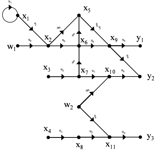
Figure 1. Digraph associated to system of Example 2
