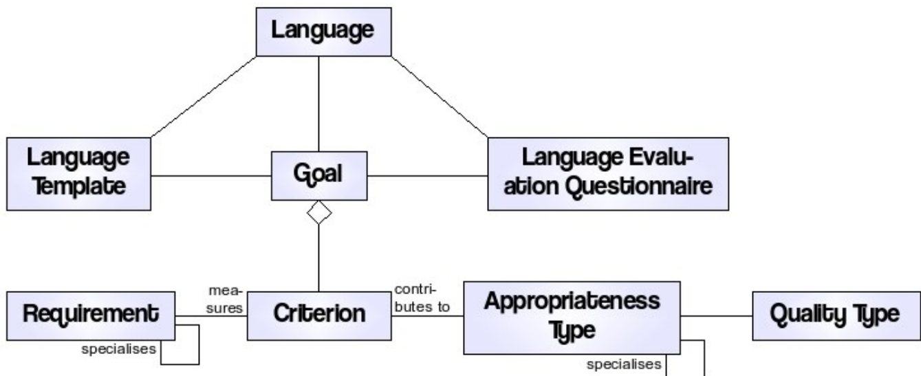
Figure 3: The UEMML language quality framework.
