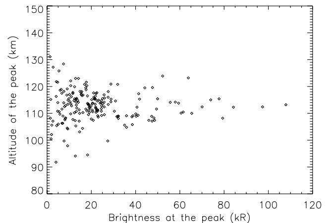
Figure 10. Relationship between the tangent point altitude of the emission peak and its brightness.
