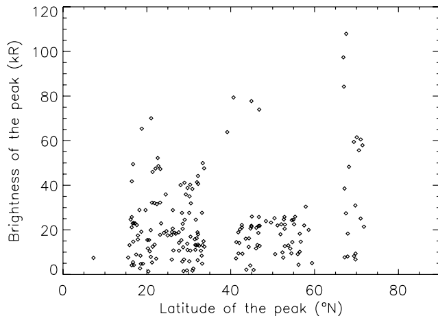
Figure 9. Relationship between the brightness of the emission peak and its latitude.
