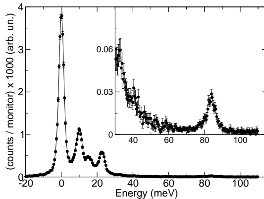
FIG. 1: Inelastic x-ray scattering example spectrum of \text{La}_{1.86}\text{Ba}_{0.14}\text{CuO}_{4+\delta} , at \mathbf{Q} = (3.11, 0.04, 0) (see text).
