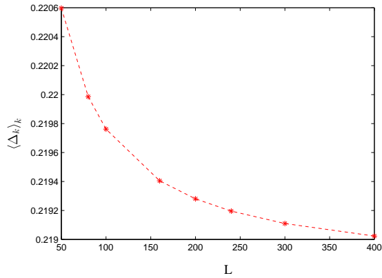
FIG. 7: (Color online) Evolution of \langle \Delta_k \rangle_k as a function of the number of points in the Brillouin zone
