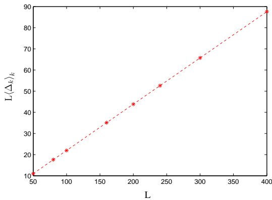
FIG. 8: (Color online) Evolution of L \times \langle \Delta_k \rangle_k as a function of the number of points in the Brillouin zone.
