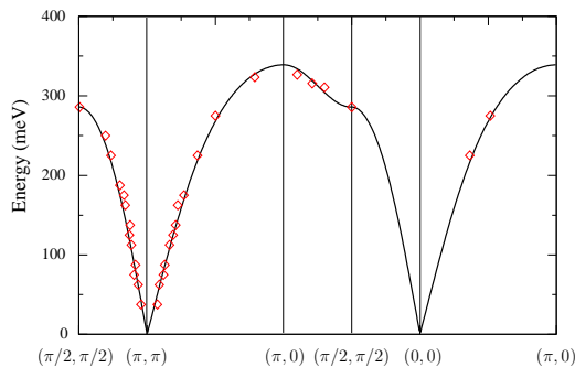
FIG. 4: (Color online) Magnon energy in \text{La}_2\text{CuO}_4 , as a function of wave vector \mathbf{k} , across the Brillouin zone at a temperature of 10 K. The experimental data (red squares) are from reference 6 . The fit is made using the parameters given by (38).
