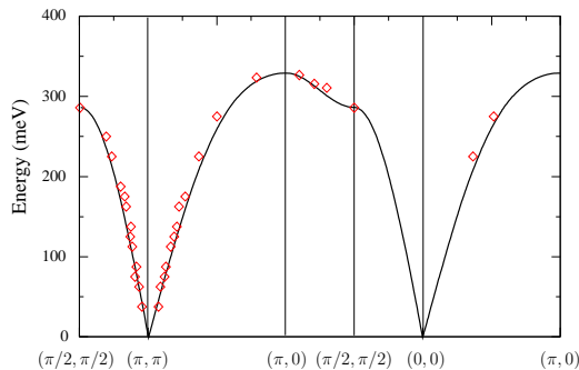
FIG. 3: (Color online) Magnon energy in \text{La}_2\text{CuO}_4 , as a function of wave vector \mathbf{k} , across the Brillouin zone at a temperature of 10 K. The experimental data (red squares) and fit (full line) are from reference 6 . The \{t, t', t'', U\} fitting parameters are given in (36).
