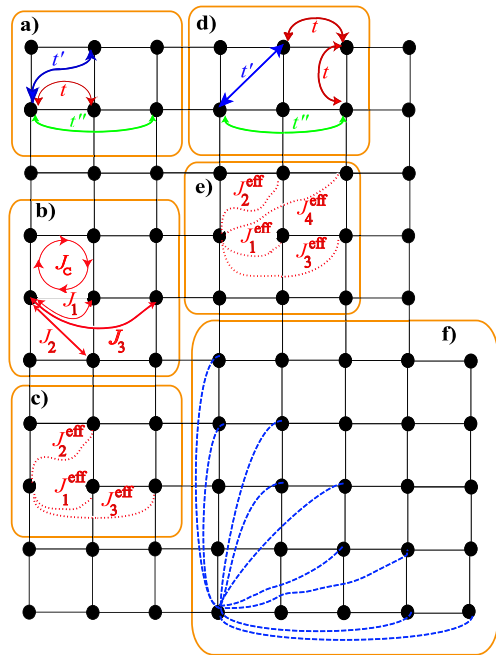
FIG. 1: (Color online) Hopping processes and resulting spin interactions. a) shows the different hopping processes characterized by parameters t , t' and t'' in the Hubbard model considered in this paper. t , t' and t'' are hopping parameters between first, second and third nearest neighbors, respectively. b) At half-filling, and when t' = t'' = 0 , canonical perturbation theory leads to order t^4/U^3 to an effective spin-1/2 Hamiltonian, H_s^{(4)} , characterized by first ( J_1 ), second ( J_2 ) and third ( J_3 ) nearest neighbor exchange interactions as well as a 4-spin ring (cyclic) exchange interaction with coupling strength J_c . c) In a large S expansion, H_s^{(4)} can be recast to order 1/S as an effective spin Hamiltonian which only involves bilinear (pairwise) spin-spin exchange interactions between first ( J_1^{\text{eff}} ), second ( J_2^{\text{eff}} ) and third ( J_3^{\text{eff}} ) nearest neighbors. To order 1/S , the effect of the ring exchange of strength J_c merely renormalizes the first and second nearest-neighbor exchange as discussed in Ref. [6]. d) illustrates an example of a four hops (ring exchange) electronic process that involves t' and t'' and contribute to order t^2 t' t'' / U^3 to the spin Hamiltonian H_s^{(4)} . e) shows that the ring exchange term illustrated in d) introduces in the 1/S approximation of H_s^{(\text{eff})} a fourth nearest neighbor exchange, J_4^{\text{eff}} as well as renormalize the J_1^{\text{eff}} , J_2^{\text{eff}} and J_3^{\text{eff}} of c) . f) illustrates all the additional J_n^{\text{eff}} exchanges beyond those shown in c) and which are generated by all the hopping processes involving an allowed combination of t , t' and t'' to order 1/U^3 .
