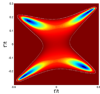
(b) \chi^2 with odd powers of t'/t and t''/t included
