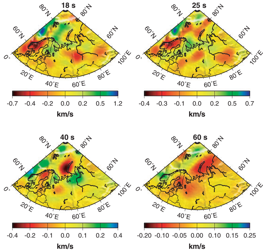
Figure 6. Difference between the initial and newly inverted group-velocity maps of Love waves with period of 18, 25, 40 and 60 s (in \text{km s}^{-1} ).
