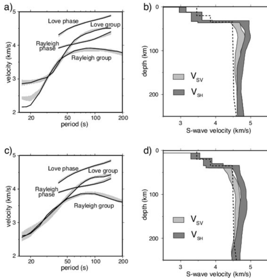
Figure 10. Examples of the inversion for acceptable 1-D shear velocity models. (a) and (b) A point in the Barents Sea (74°N, 40°E). (c) and (d) A point in Western Siberia (70°N, 70°E). (a) and (c) Four dispersion curves obtained from tomographic velocity maps (thick black lines) and the predictions from the ensemble of acceptable models (grey lines) shown in (b) and (d), respectively. (b) and (d) The ensemble of acceptable models where SV and SH velocities are presented with light and dark grey shades, respectively. The corridor of acceptable values is indicated by the solid black lines. The S-wave velocity from the global reference model ak135 (Kennett et al. 1995) is plotted as the dash line.
