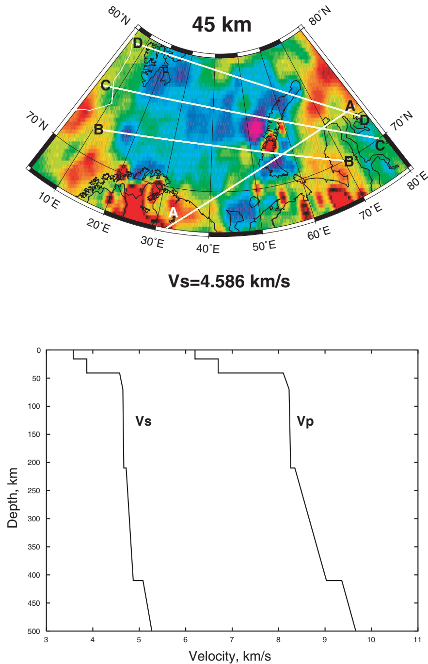
Figure 12. Results of the 3-D tomographic inversion: isotropic shear wave velocities V_s = (V_{sv} + V_{sh})/2 at 45 km relative to the 1-D model Barey (top). The map contains in addition the position of the different transects through the model as shown in Fig. 13. The Barey model (Schweitzer & Kennett 2002) used in this study as 1-D reference model is shown at the bottom.
