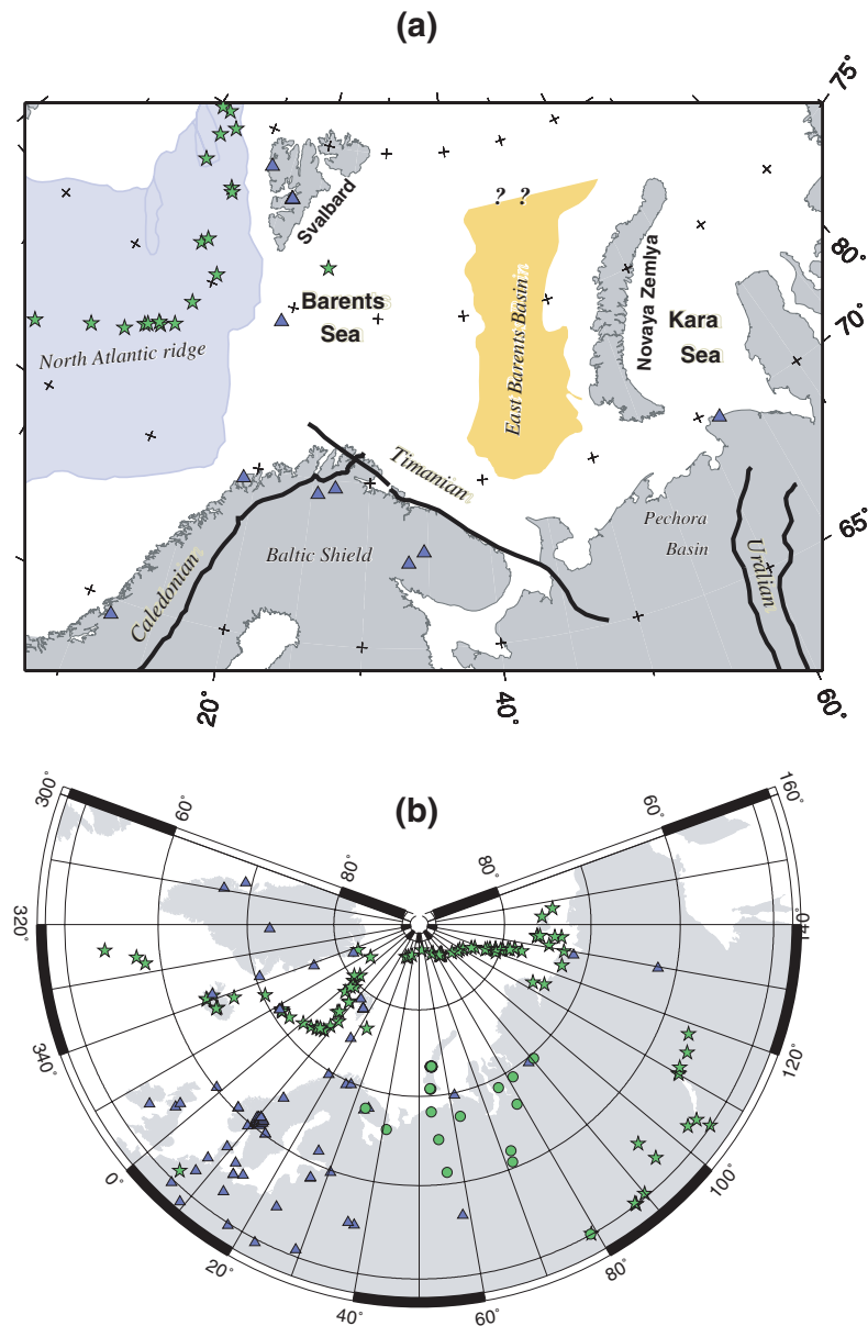
Figure 1. (a) The map shows the most relevant tectonic features discussed in the text. Blue shaded regions depict the north Atlantic oceanic domain, outlining the continent–ocean boundary in the European Arctic and the Norwegian Sea. The yellow shaded area in the East Barents Sea marks sediment thicknesses larger than 9 km in the East Barents Sea basin, after Johansen et al. (1992). Note that the geometry in the northern part of the basin is uncertain as indicated by question marks. The mid-Atlantic ridge is traced by the epicentres (green stars) and stations used in this study are displayed by blue triangles. (b) The map shows the location of the seismic stations (blue triangles) and events used in this study (see also Table 1). The epicentres of the earthquakes are shown by green stars, explosions as green circles.
