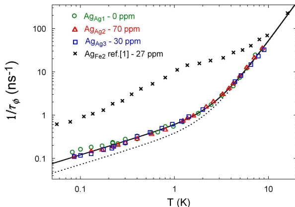
FIG. 3: Inverse of the phase coherence time as a function of temperature for samples Ag_{Ag1} , Ag_{Ag2} and Ag_{Ag3} as well as Ag_{Fe2} from ref. 1 . The solid line is the best fit to equation 2. The dotted line is the theoretical expectation for sample Ag_{Ag1} .
