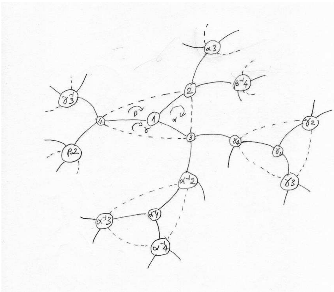
Universal cover and tessellation of K_4
