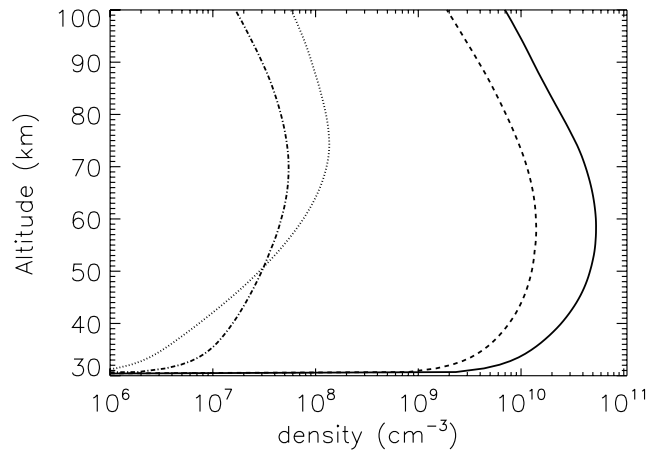
Figure 13. O and N density profiles. The solid line and the dotted line are the oxygen and the nitrogen density profiles from orbit 716 respectively. The dashed line and the dotted-dashed line are the oxygen and the nitrogen density profiles deduced from orbit 1577, respectively.
