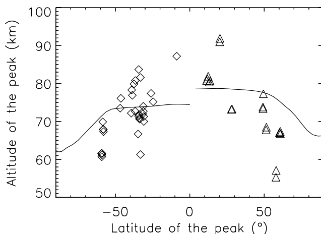
Figure 5. Variation of peak altitudes as a function of latitude. Diamonds are data of L_s = [35, 75]^\circ and triangles are data of L_s = [185, 225]^\circ . The black lines represent the 0.1 Pa isobars for L_s = 40^\circ (left) and L_s = 190^\circ (right).
