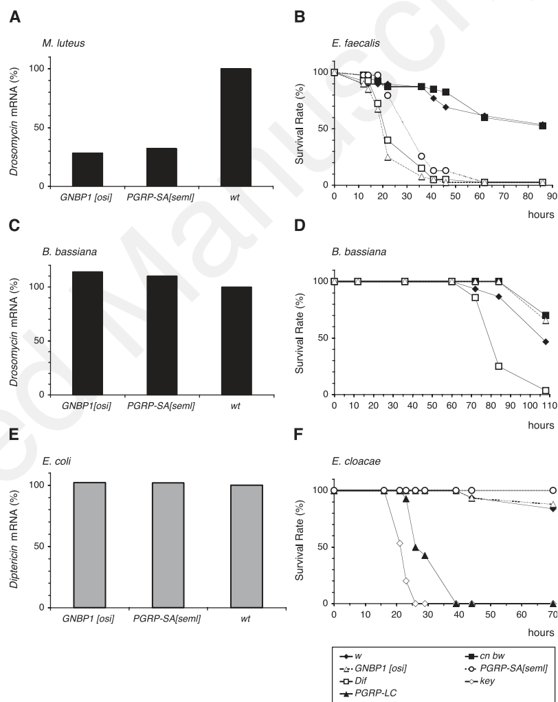
Fig. 1. GNBP1 is required for the host response against Gram-positive bacteria and not for that against Gram-negative bacteria or fungi. (A and C) Representative values for Drosomycin mRNA steady-state levels as measured by quantitative–reverse transcription–polymerase chain reaction (Q-RT-PCR) (supporting online material). The panel shows the induction of Drosomycin mRNA after an immune-challenge with (A) Micrococcus luteus (for 24 hours, at 20°C) or (C) B. bassiana (for 36 hours, at 25°C) in GNBP1 osi ( GNBP1 osi ), PGRP-SA seml ( PGRP-SA seml ), and wild-type (wt) control flies. The level of inducibility measured in the wild type was arbitrarily set to 100, and the measures obtained in the mutants were expressed as a percentage of this value. (B, D, and F) Survival experiments. We monitored the survival rate (expressed in percentage) after immune challenge. As expected, Dif mutant flies died more rapidly than wild-type (w) controls after (B) Gram-positive ( E. faecalis , at 25°C) and (D) natural fungal ( B. bassiana , at 29°C) infections, whereas (F) IMD pathway mutants kenny ( key ) (25) and PGRP-LC ET12 (26) succumbed rapidly to E. cloacae (at 25°C) infection. The Dif and key mutations were originally generated in the cn bw genetic background, which serves as a wild-type control. (E) Diptericin mRNA levels 6 hours after an immune challenge at 20°C with Escherichia coli in GNBP1 osi , PGRP-SA seml , and wild-type flies.
