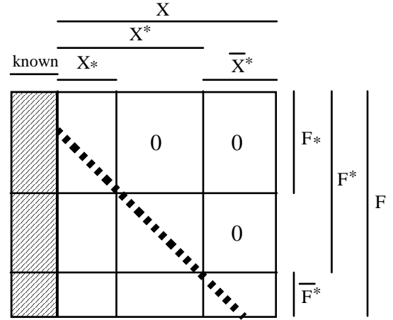
Fig. 1: Canonical decomposition
