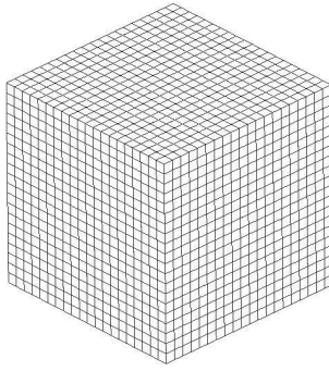
Fig. 4. Cube under traction: mesh for problem 1 (2400 elements).
