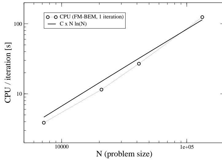
Fig. 6. Cube under traction: CPU times per iteration for the FM-BEM, and best fit of the form CPU=C \times N \ln N , with C \approx 7.92 \cdot 10^{-5}s .
