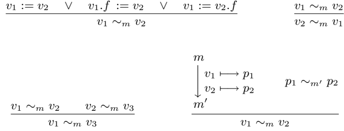
Fig. 1. The Pointer Interference Algorithm
