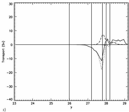
FIG. 5. (a) Surface dianeutral fluxes poleward of 30°S (Sv): total transport (solid line), the heat component (dashed line), and the freshwater component (dotted line). The vertical lines are the water-mass boundaries in Table 1. As in the classical formulation, positive (negative) values indicate that surface fluxes are transforming surface water into higher (lower) density classes. (b) Values for the region between 42°S and Antarctica. (c) Surface dianeutral fluxes at the ice-ocean interface.
