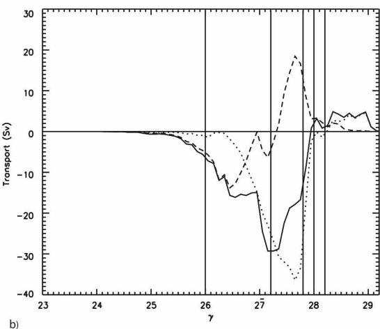
FIG. 6. Surface dianeutral fluxes (dashed line), net transformations at 30°S (solid line), and dianeutral fluxes due to mixing processes (dotted line) (Sv).
