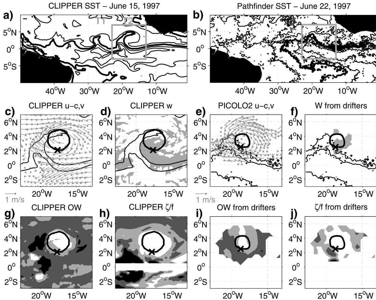
FIG. 1. (a) CLIPPER model SST averaged from 13 to 17 Jun 1997 at a 1°C contour interval, with the 25.5 contour in thick black; colder temperatures are found at the equator. (b) Pathfinder AVHRR SST on 22 Jun 1997, with the same contours as in (a). (c), (e) Zoom, respectively, on square regions indicated in (a) and (b), showing CLIPPER and Pathfinder 24° and 25.5°C SST contours (black thin solid line), CLIPPER and PICOLO drifter surface velocity vectors (gray arrows) in a frame of reference moving westward at 32 cm s -1 , and a closed streamline (thick solid black). The black star indicates the starting point of the vertical sections shown in Fig. 4. (d), (f) Respectively, positive vertical velocity in CLIPPER and PICOLO from drifter velocity in gray shading, with 24° and 25.5°C CLIPPER and Pathfinder SST contours. (g), (i) Respectively, Okubo–Weiss parameter in CLIPPER and PICOLO from drifter velocity in gray shading, with contours of -5 \times 10^{-10} , 0, 5 \times 10^{-10} s -2 from white to black. (h), (j) Respectively, the ratio of relative to planetary vorticity in CLIPPER and PICOLO from drifter velocity in gray shading, with contours of -0.5, 0, and 0.5 from white to black. Values of -1 are reached within the vortex.
