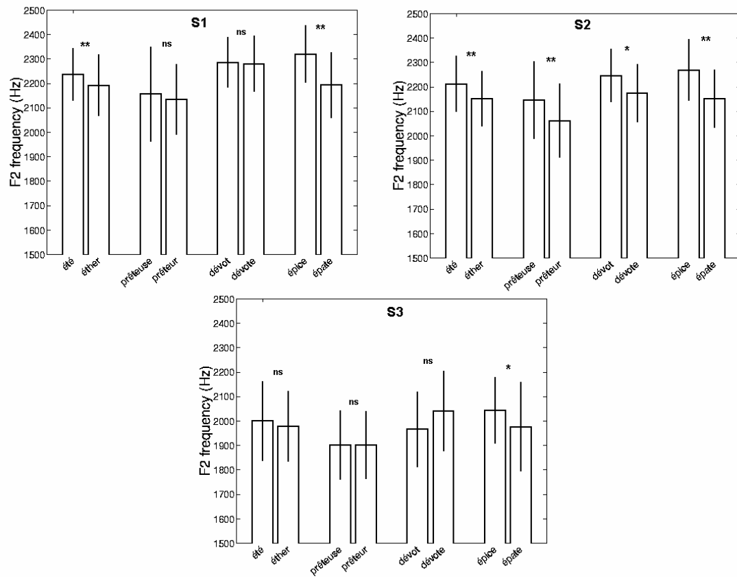
Figure 1. Mean F2 values and standard deviations for four sets of words containing a word-initial mid front vowel [e], and followed by the vowels [e]/[ɛ], [o]/[ɔ], [ø]/[œ], and [i]/[a] for two Parisian (S1 and S2) and one Southern (S3) female speakers (** significant at p < 0.01 , * significant at p < 0.05 , ns non-significant).
