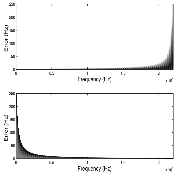
Figure 1: On top, estimation error of f^- versus the frequency of the analyzed sinusoidal signal. At bottom, estimation error of f^+ . It appears that the errors of these two estimators are symmetrically distributed around frequency F_s/4 .
