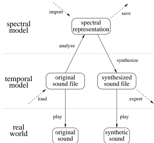
Figure 1: InSpect Architecture
