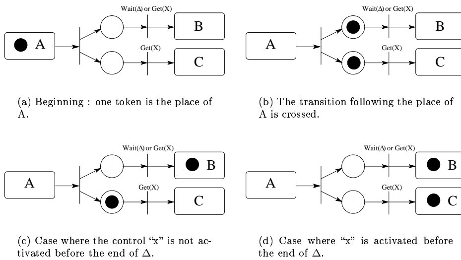
Figure 14: The evolution of the Petri Network associated to a black arc
