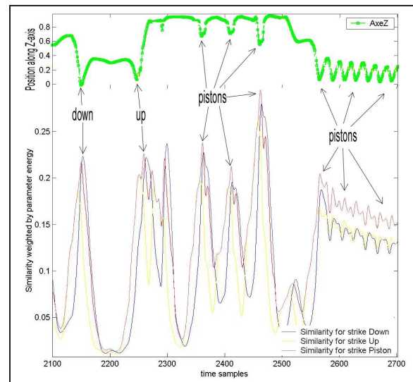
Figure 6. A sample of play with position information (top) and similarity to each strike type (bottom).
