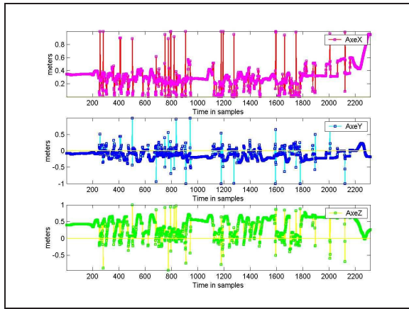
Figure 1. The FOB may deliver very disturbed signals depending on the electromagnetic environment.
