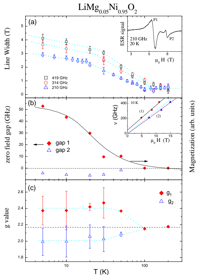
FIG. 7: (Color online) ESR spectra parameters for Mg doped \text{LiNiO}_2 as a function of temperature.
