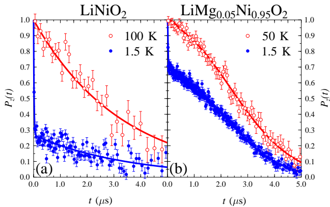
FIG. 2: (Color online) Corrected asymmetry [ P_z(t) ] data at high and low temperature for: (a) \text{LiNiO}_2 with fits to Eq. 1 using the parameters shown in Fig. 3, and (b) 5 % Mg-doped sample with fits to Eq. 2 using the parameters shown in Fig. 4. For clarity of display the histogram binning has been altered and the data sets have been normalized with a temperature independent background subtracted.
