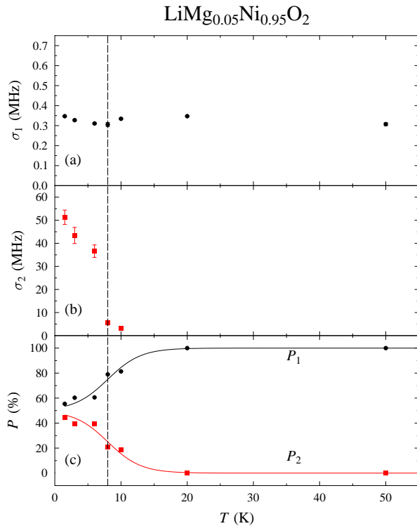
FIG. 4: (Color online) Parameters derived from fitting Eq. 2 to the raw positron asymmetry data for 5 % Mg-doped \text{LiNiO}_2 . (a) \sigma_1 describing the slower relaxing component. (b) \sigma_2 describing the faster relaxing component. (c) Amplitudes of the relaxation components P_1 and P_2 . The lines are guides to the eye.
