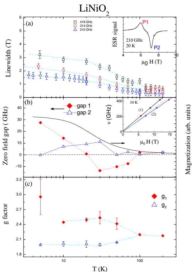
FIG. 6: (Color online) ESR spectra parameters for quasi stoichiometric \text{LiNiO}_2 as a function of temperature.
