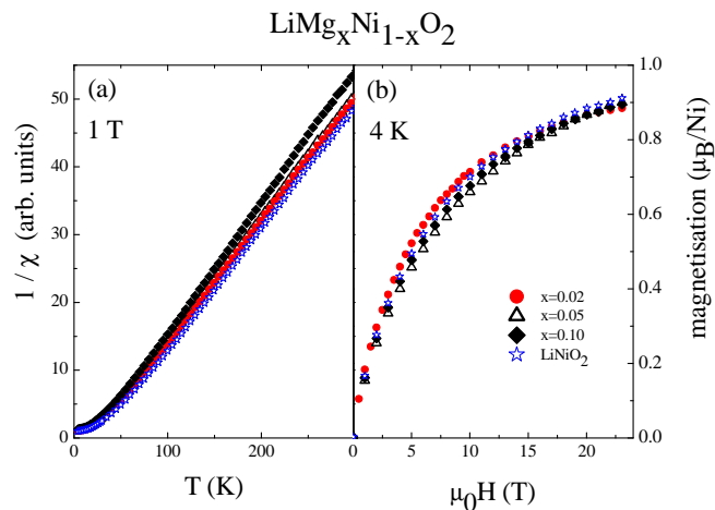
FIG. 1: (Color online) Magnetic properties normalized per Ni ion for quasi-stoichiometric LiNiO _2 and LiMg _x Ni _{1-x} O _2 with x=0.02, 0.05 and 0.10 . (a) Inverse of the susceptibility at 1T as a function of temperature. (b) Magnetization at 4K as a function of magnetic field.
