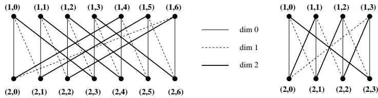
Fig. 1. W_{14,3} and (right) W_{8,3}
