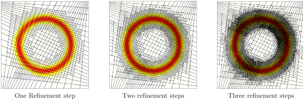
FIGURE 19. Quadrangle- Q_1 . Refined meshes.
