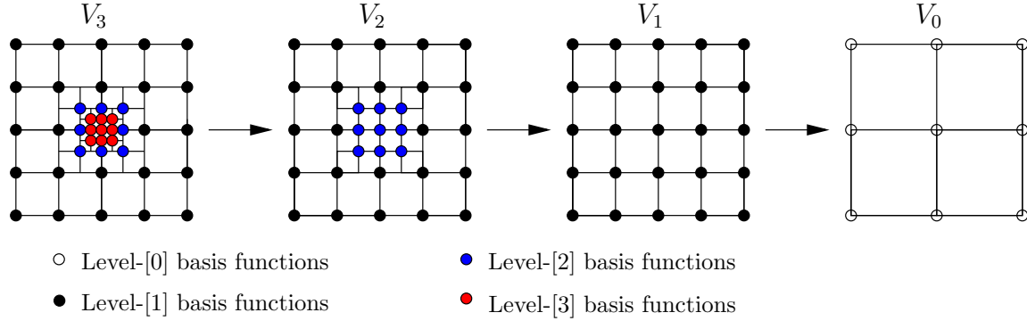
FIGURE 13. Example of coarsening : from V_3 to V_0 .
