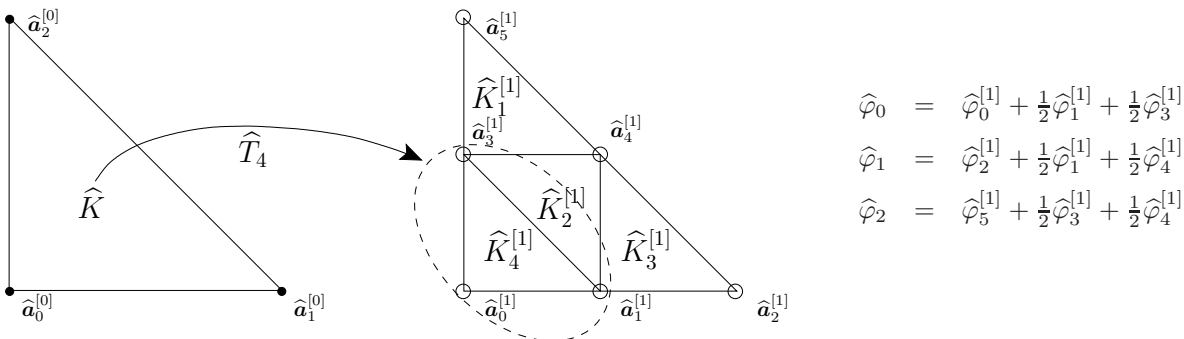
FIGURE 5. \mathbb{P}_1 -triangle refinement pattern and refinement equations.
