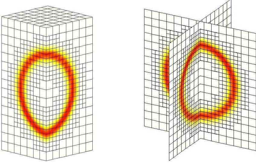
FIGURE 20. Refined mesh in 3D. One refinement step.
