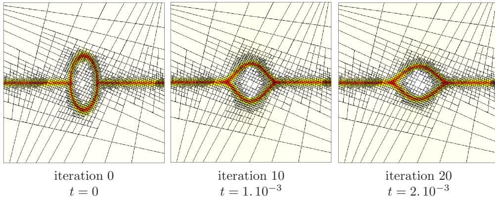
FIGURE 23. Quadrangle- \mathbb{Q}_1 . Time marching. h_{\text{interface}} = 0.8\varepsilon
