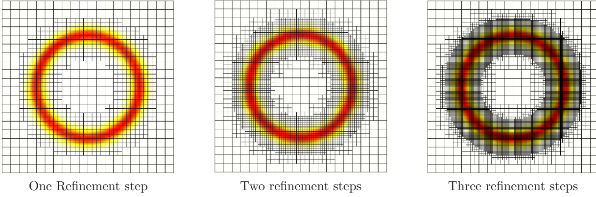
FIGURE 17. Square- Q_1 . Refined meshes.
