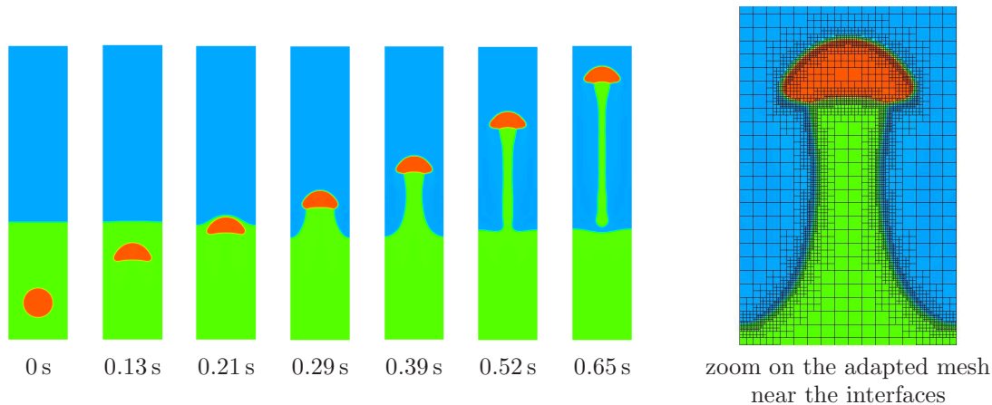
FIGURE 25. Entrainment of an heavy liquid during a bubble rising.
