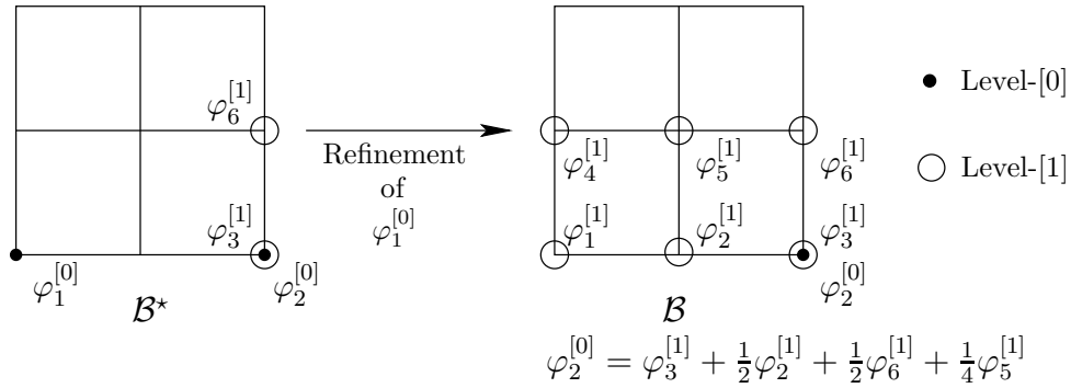
FIGURE 10. Refinement do not preserve the linear independence of multilevel set not satisfying (\mathcal{P}_{LI}) .
