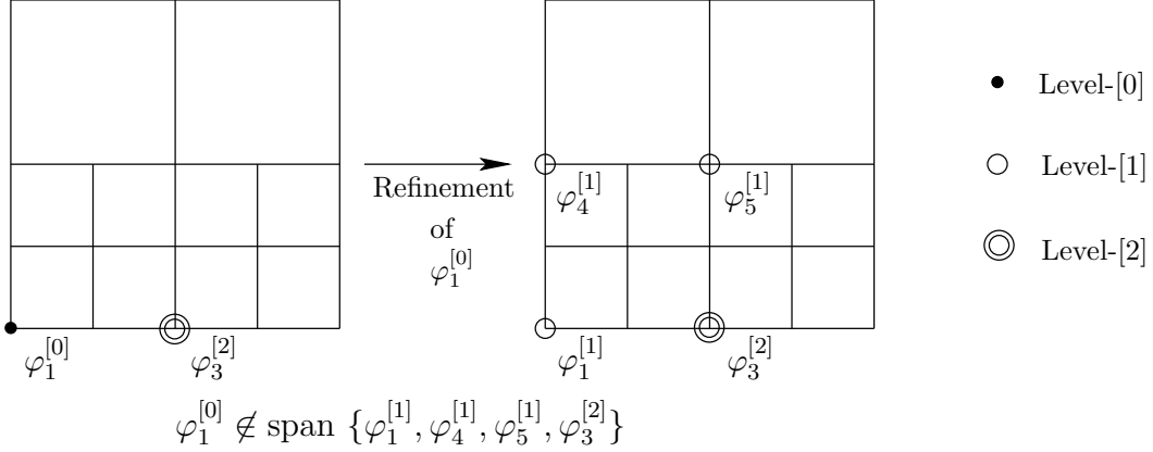
FIGURE 11. Refinement of multilevel basis is not lossless.
