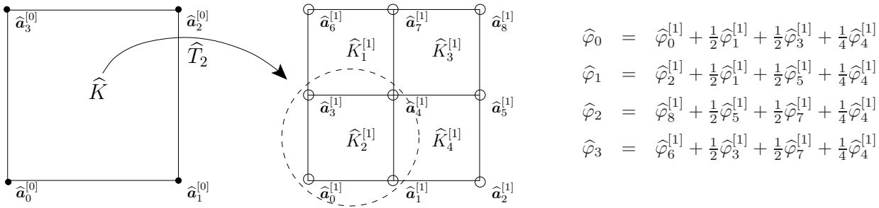
FIGURE 4. \mathbb{Q}_1 -square refinement pattern and refinement equations.
