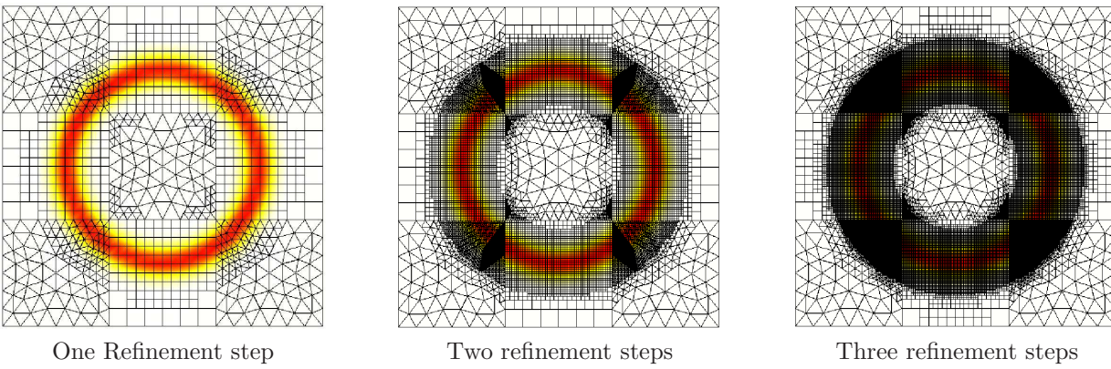
FIGURE 18. Tri/Quadr-angle- P_1/Q_1 . Refined meshes.
