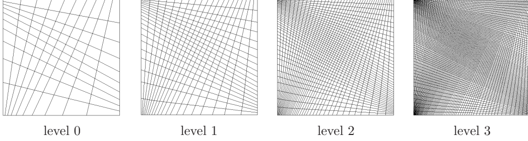
FIGURE 9. Quadrangle- \mathbb{Q}_1 . Nested meshes \mathcal{T}_j .
