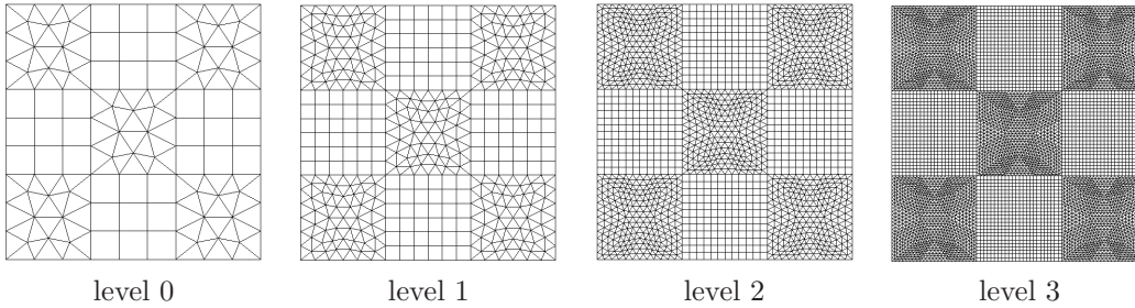
FIGURE 8. Tri/Quadr-angle- \mathbb{P}_1/\mathbb{Q}_1 . Nested meshes \mathcal{T}_j .
