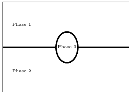
FIGURE 21. Initial position of interface. Numbering of phases.
