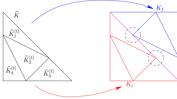
FIGURE 3. Example of an incompatible refinement pattern.
