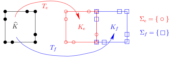
FIGURE 2. Example of incompatible node positions.
