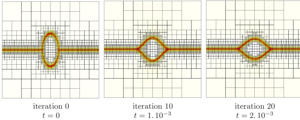
FIGURE 22. Square- \mathbb{Q}_1 . Time marching. h_{\text{interface}} = \varepsilon
