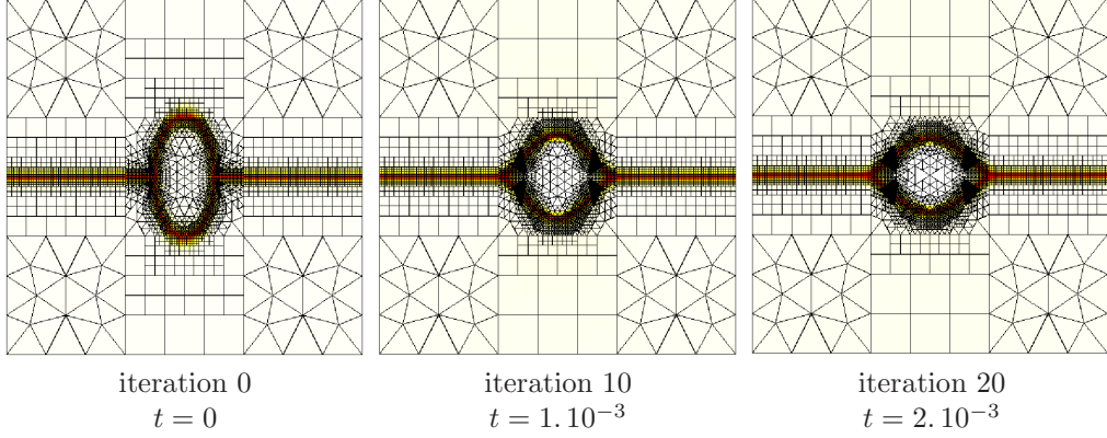
FIGURE 24. Tri/Quadr-angle- \mathbb{P}_1/\mathbb{Q}_1 . Time marching. h_{\text{interface}} = 0.4\epsilon
