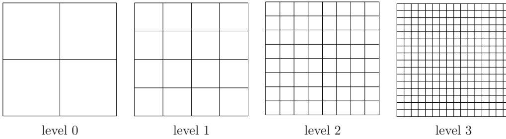
FIGURE 7. Square- \mathbb{Q}_1 . Nested meshes \mathcal{T}_j .
