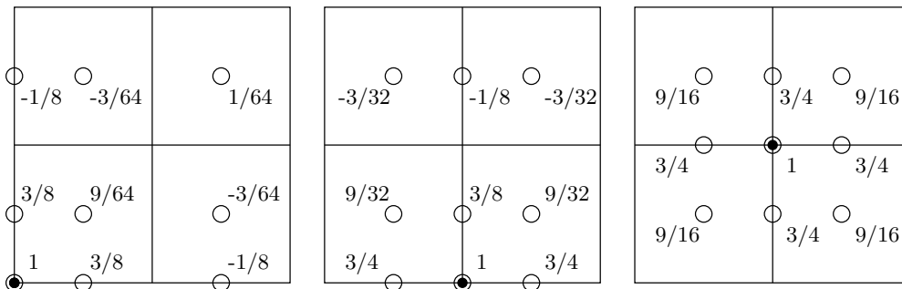
FIGURE 6. \mathbb{Q}_2 -square refinement coefficients.
