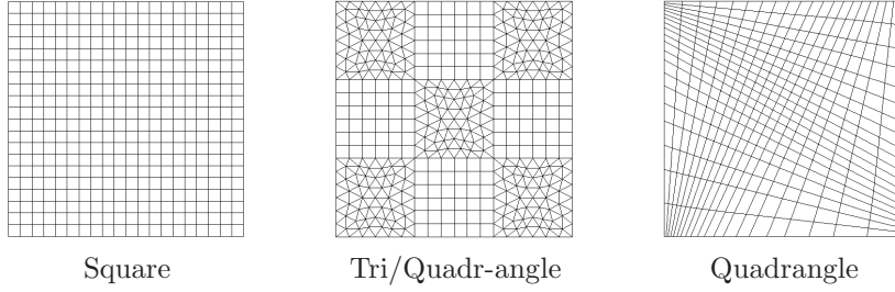
FIGURE 16. Initial meshes.
