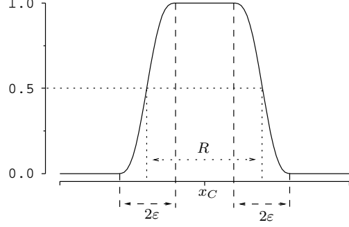
FIGURE 15. Exact solution of Problem 13, d = 1 .
