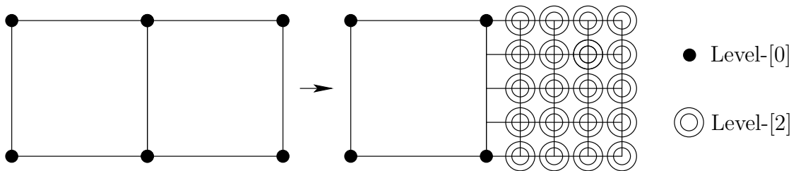
FIGURE 12. Refinement sequence forbidden by the One-level-difference rule.
