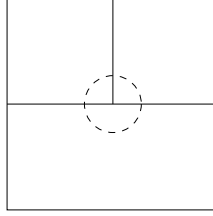
FIGURE 1. Example of a geometrically non-conformal mesh.
